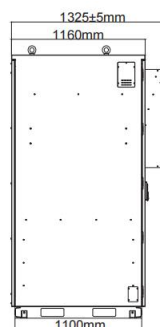
Figure 2-3 Fork position dimensions
