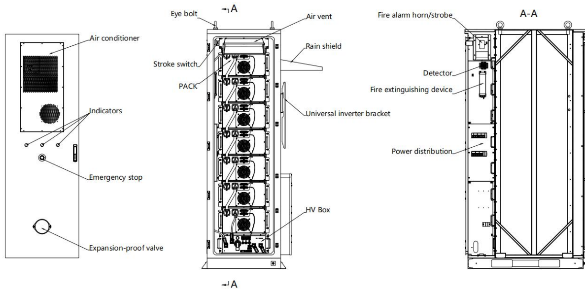
Figure 2-5 Parts description (in the closed state)
