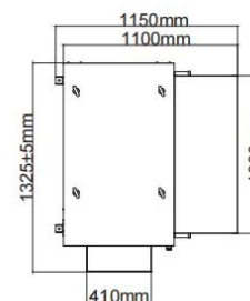
Figure 2-4 Angle supports position dimensions
