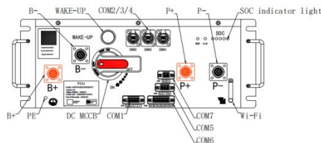
Figure 2-9 Part description
