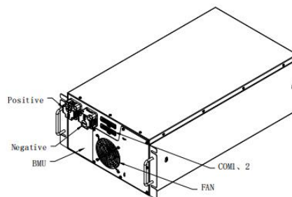
Figure 2-7 Part description
