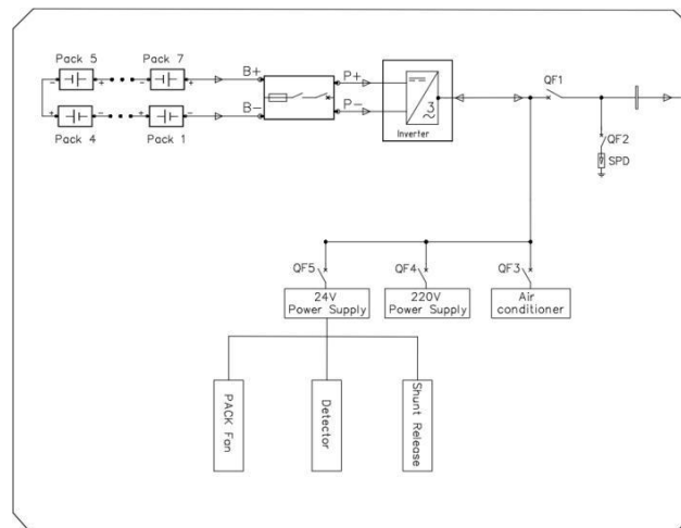
Figure 2-14 Electrical Block Diagram
