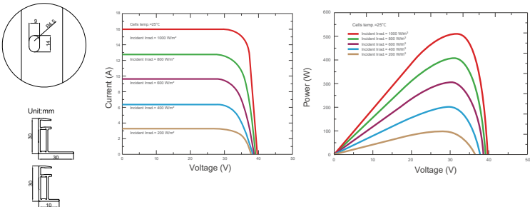
Current-Voltage & Power-Voltage Curves (SKT510M12-108D4)
